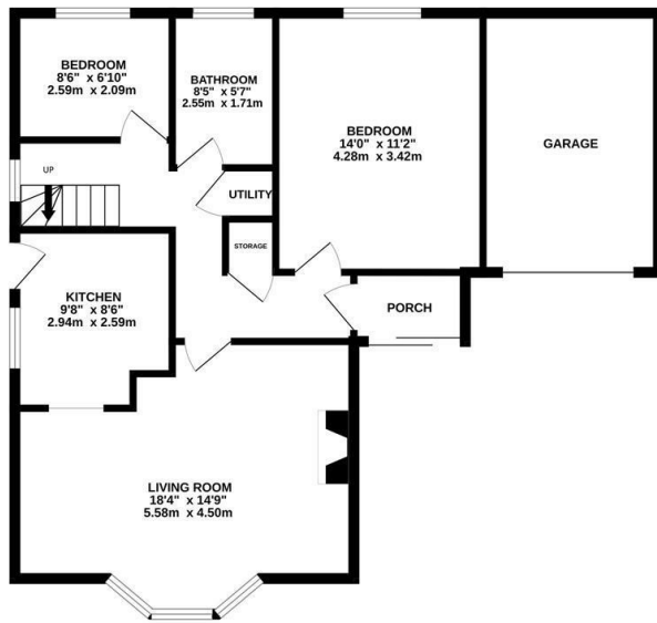
GROUND FLOOR 819 sq.ft. (76.1 sq.m.) approx.
